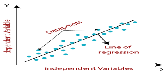
Figure 1: Linear Regression
